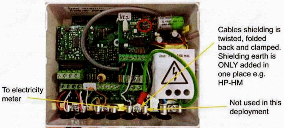
Sontex heat meter with RS485 module and mains supply
