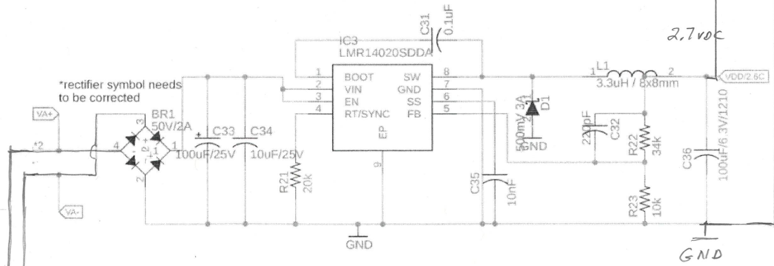
6_channel_esp32_energy_meter_1.3_rev2 Input Power Section Only
