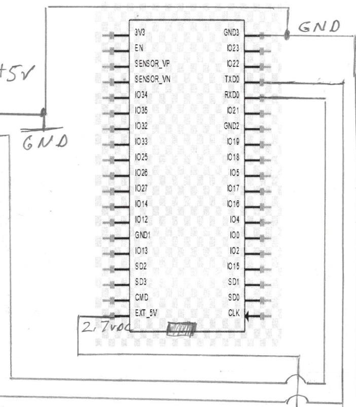
ESP32 KeeYees Wroom Connected by Header to Energy Board
